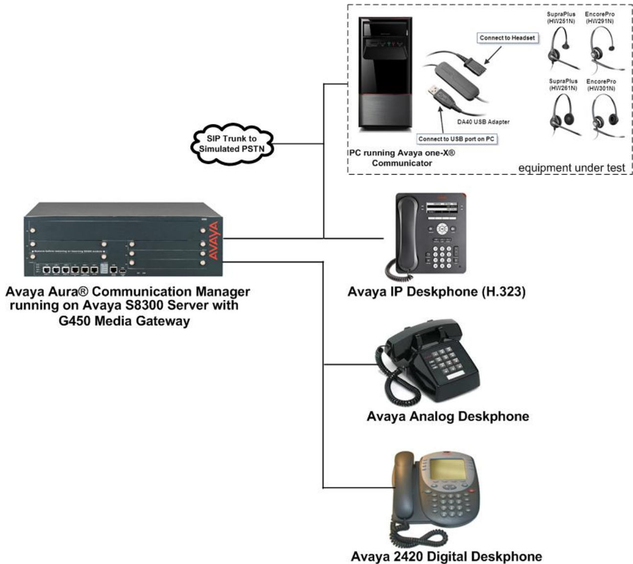
Figure 1: Avaya one-X® Communicator with Plantronics DA40 USB Adapter, Plantronics SupraPlus Wideband and EncorePro headsets.
