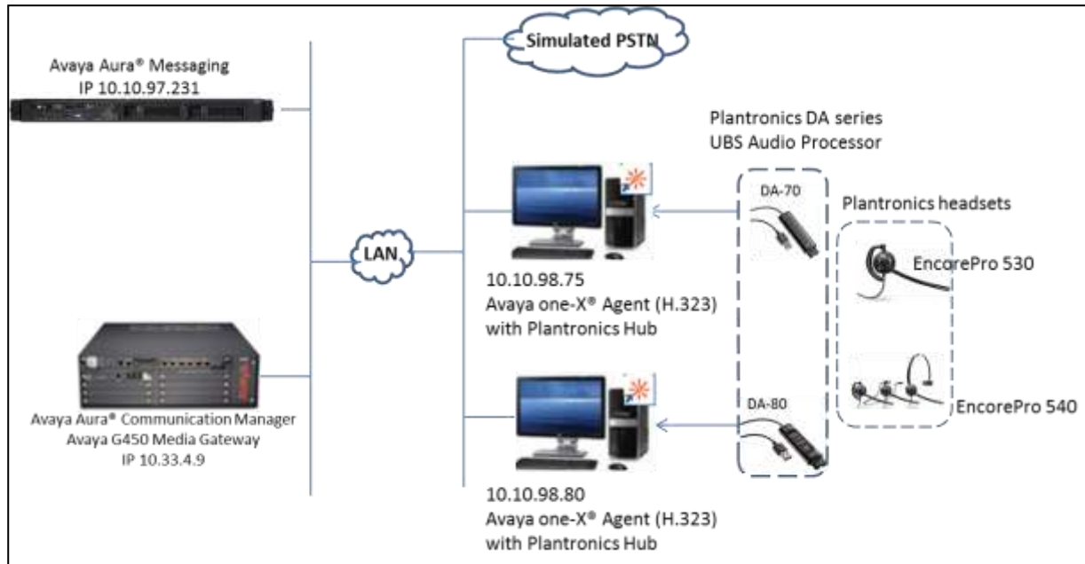
Figure 1: Test configuration
