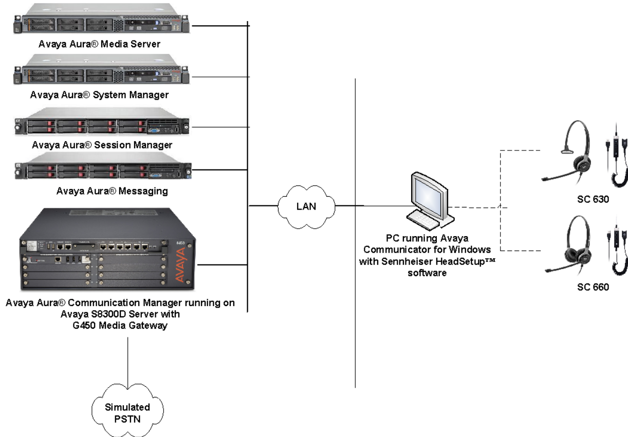
Figure 1: Test Configuration
