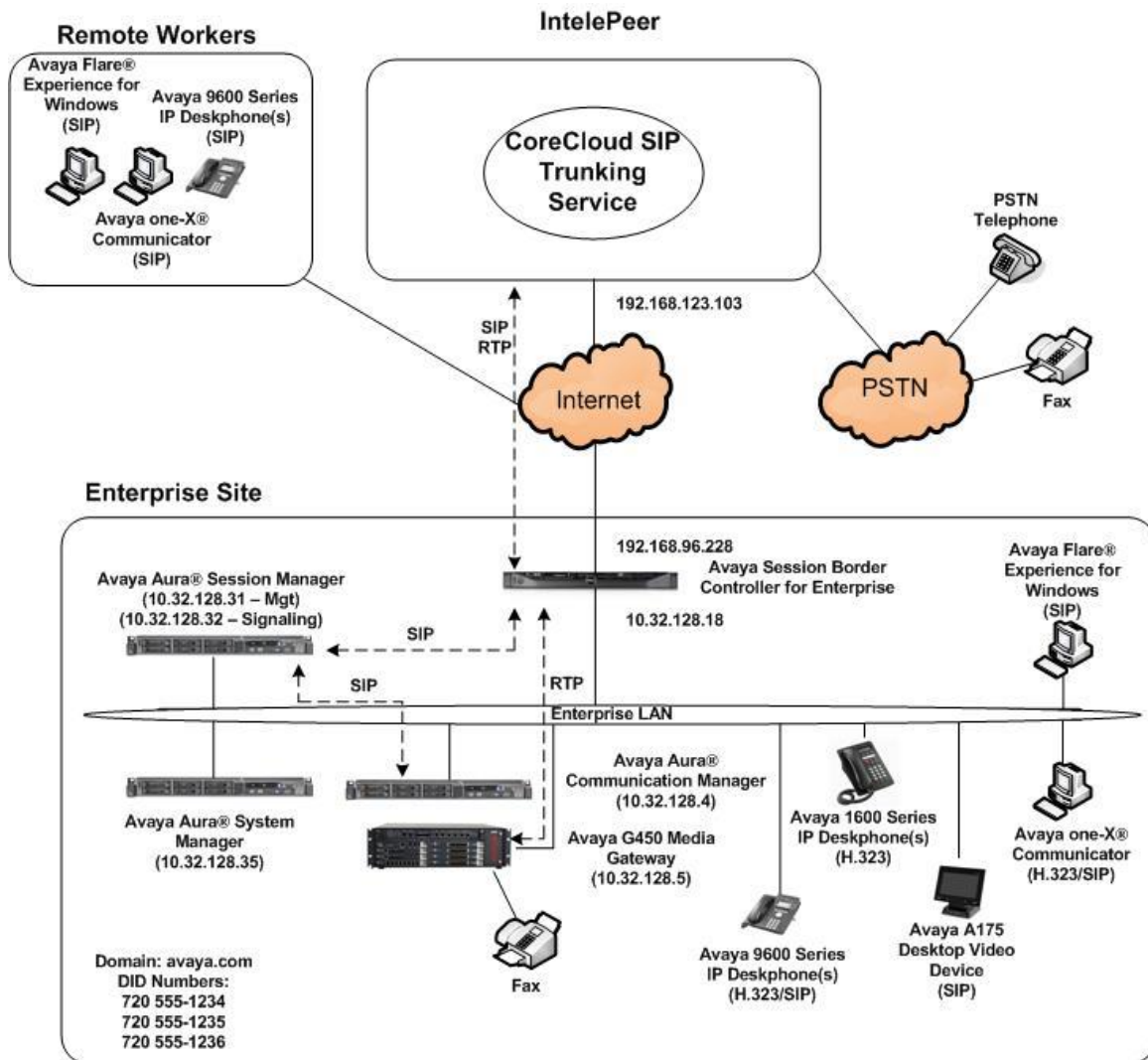
Figure 1: IntellePeer CoreCloud SIP Trunking Service Test Configuration
